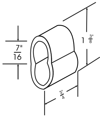
ALUMINUM SLEEVE DETAIL- B
