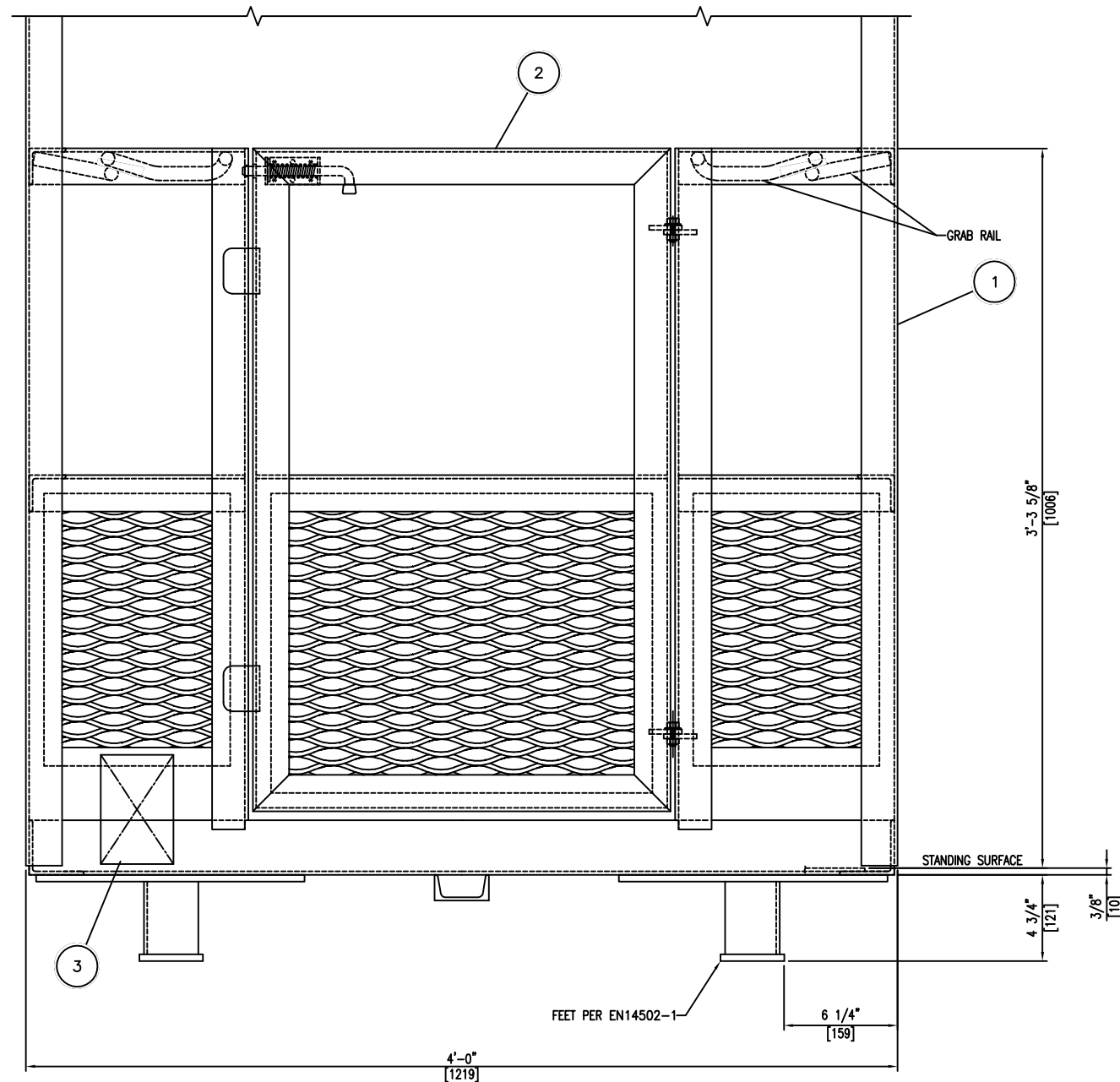
DETAIL 1 02
