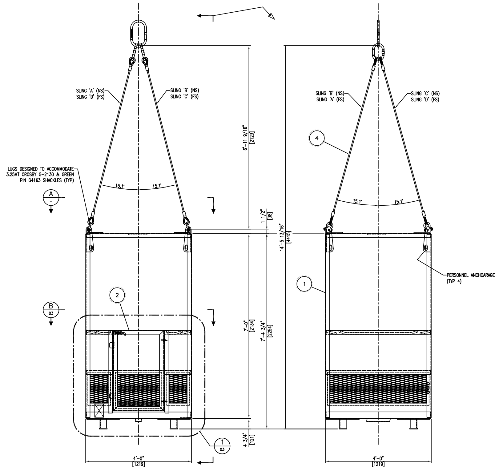
OMB-2 / EMB-2 2-MAN BASKET- ELEVATION
