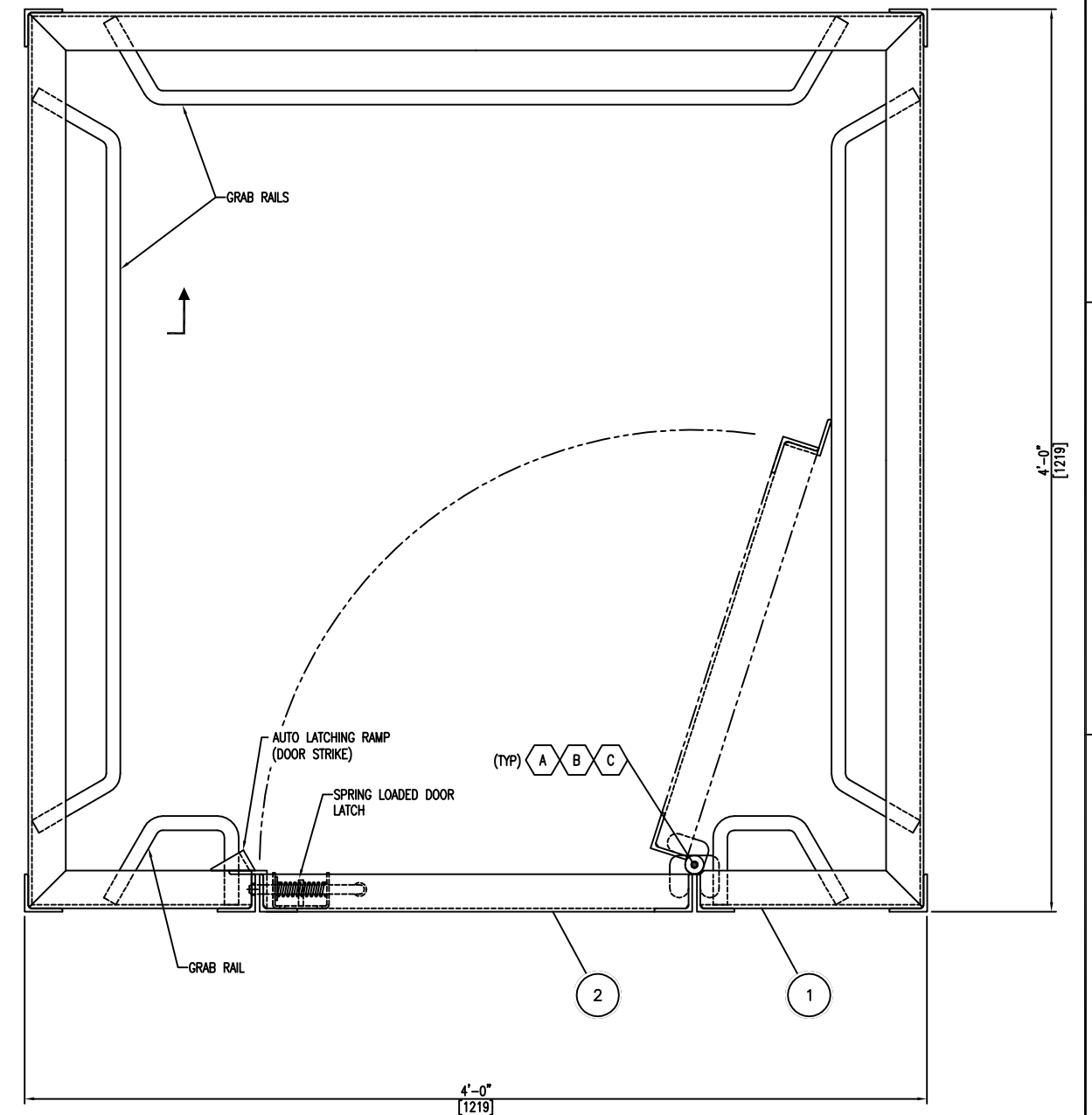
SECTION B 02
