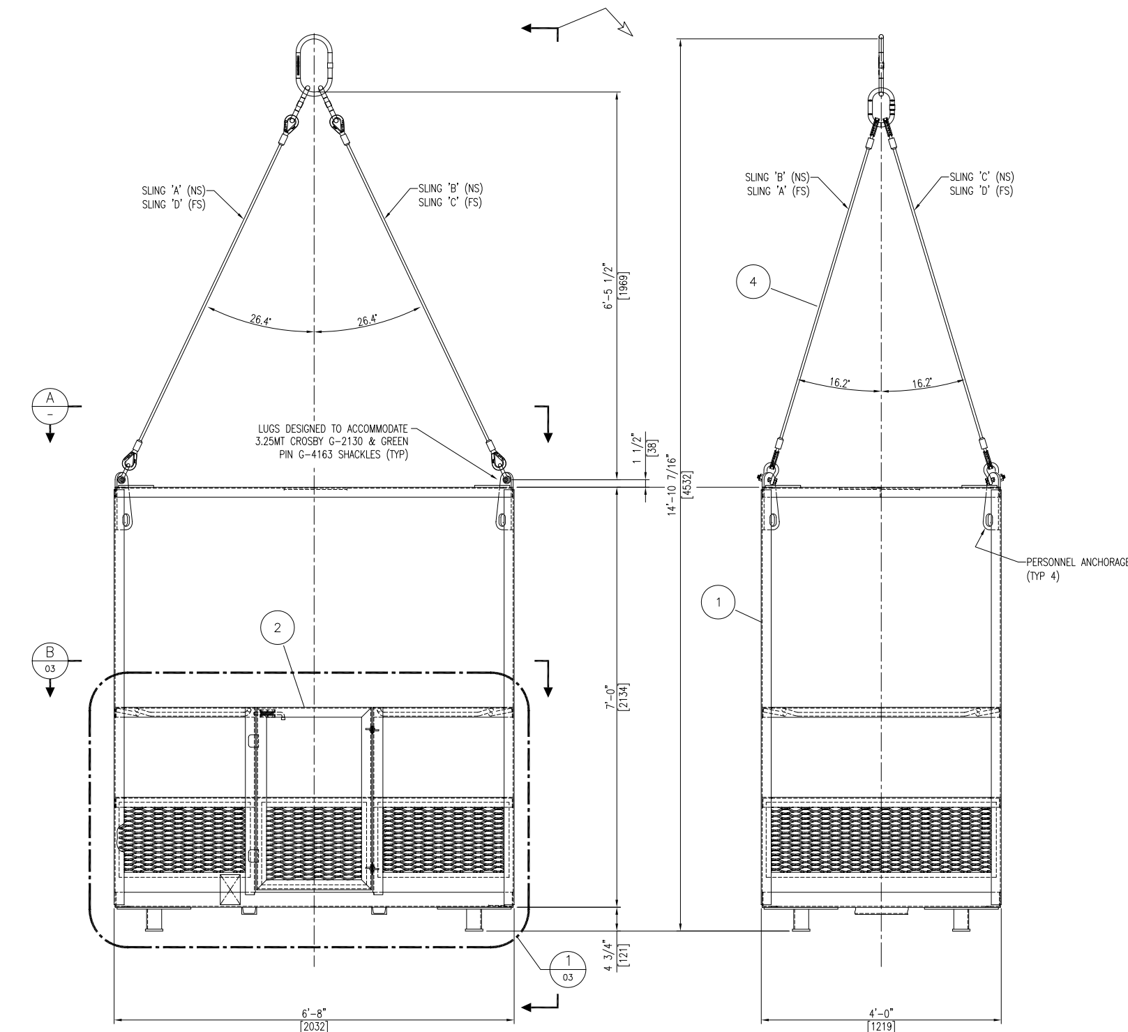
OMB-4 / EMB-4 4-MAN BASKET- ELEVATION
